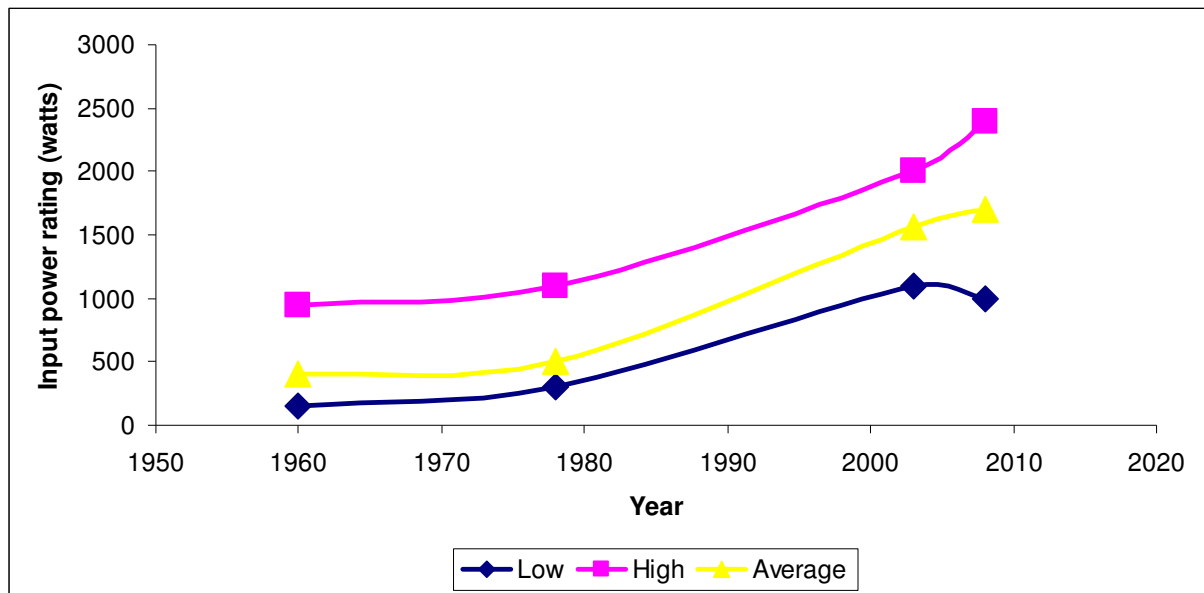
Figure 2 - Increase in Input Power Rating over Time
