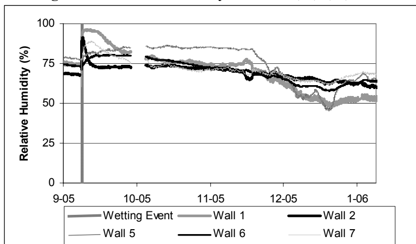
Figure 7. Relative Humidity in Walls 1, 2, 5, 6, and 7
