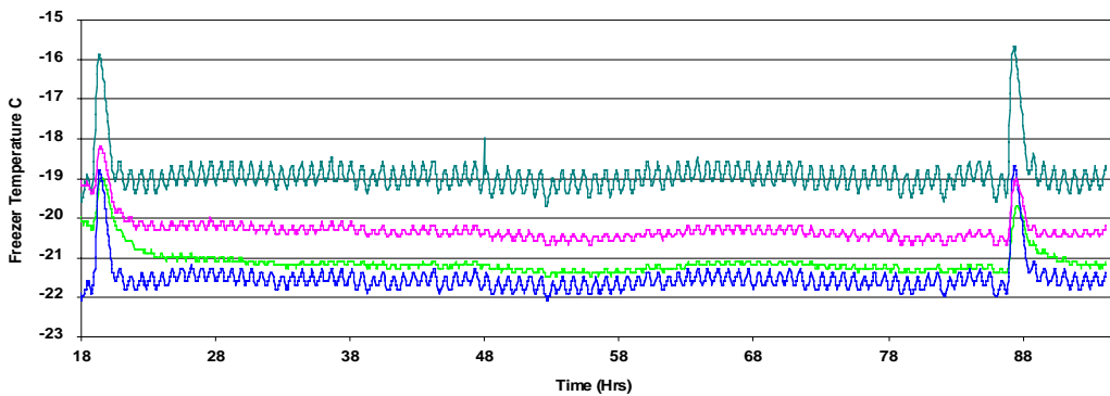
Figure 1. ISO test (25°C) showing 4 individual freezer test pack temperatures
