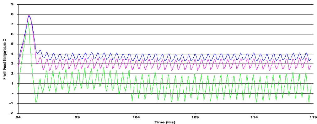
Figure 4. AS/NZS test (32°C) showing 3 individual fresh food air temperatures
