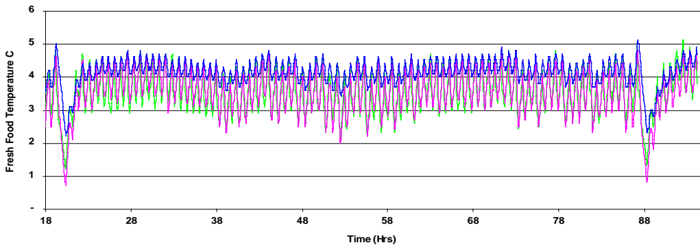
Figure 2. ISO test (25°C) showing 3 fresh food air temperatures
