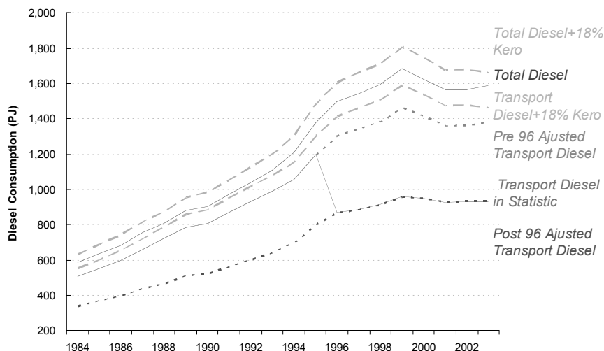
Figure 10. Top-down Estimates of Indian Transport Diesel Consumption Based on Statistics
