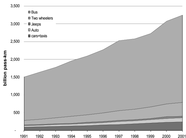
Figure 3. Road Passenger Transportation Mobility Vehicle Type
