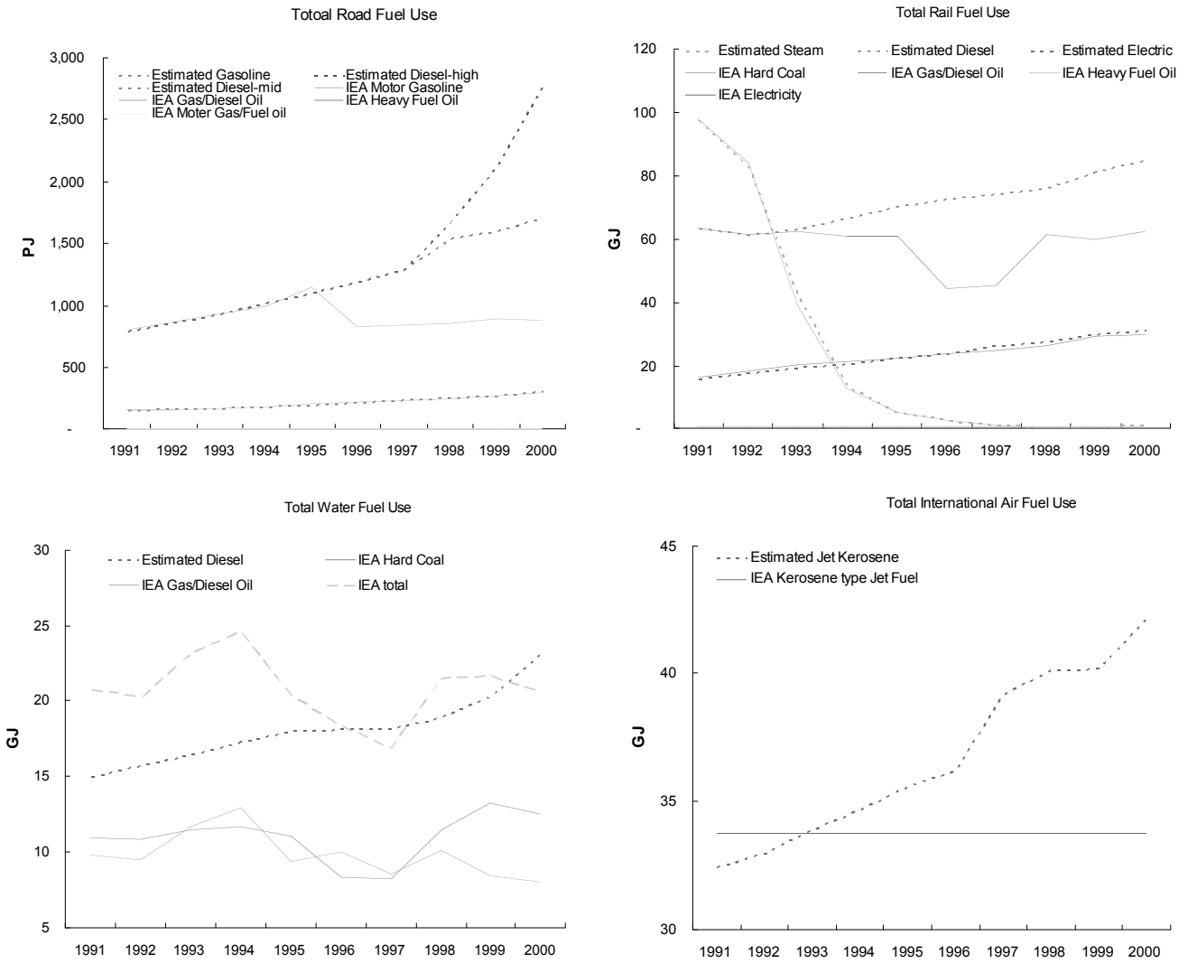
Figure 11. Comparison of the Estimated and IEA Transport Energy Use in India
