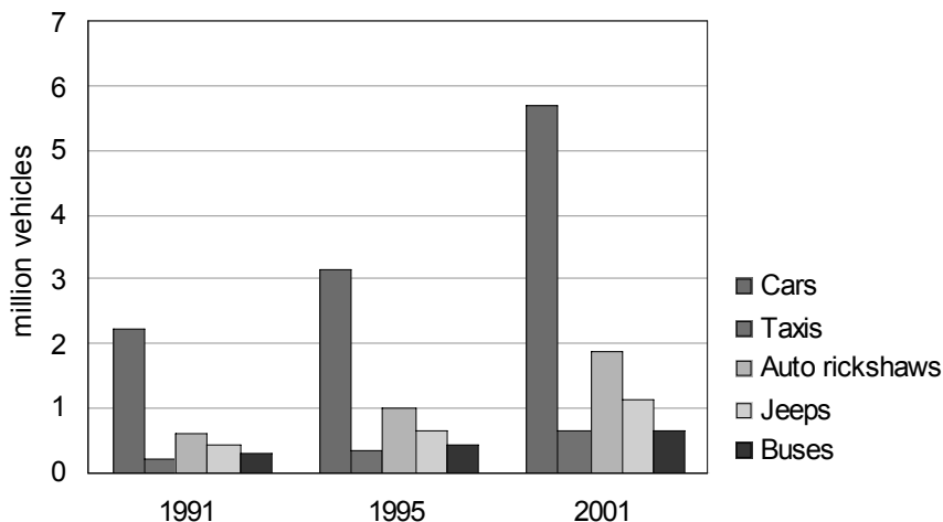
Figure 7. Change in Vehicle Stock
