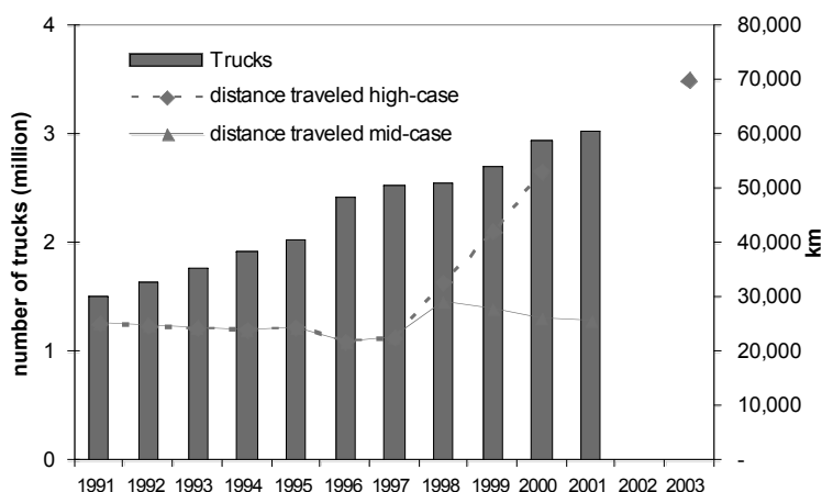
Figure 9. Change in Truck Stock and Utilization
