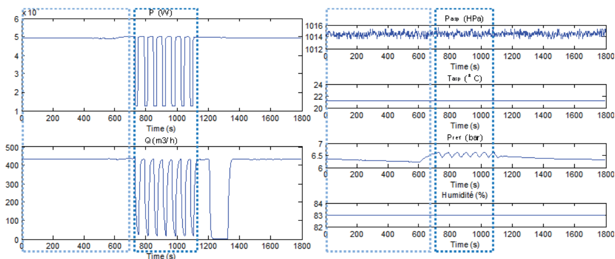
Figure 10. Relation between compressor power and compressed air flow rate (and additional parameters).
