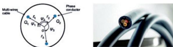
Figure 3. Cross section geometry of a typical industrial three-conductor power cable.
