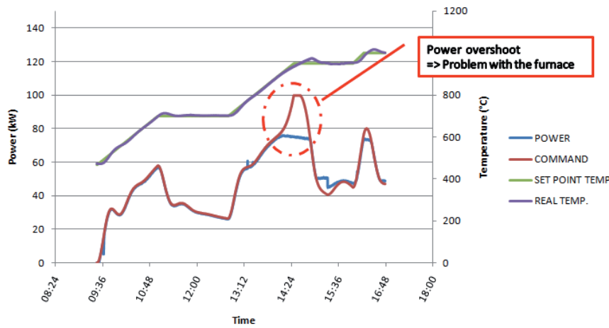
Figure 7. Power, command and inside temperature for one of EDF R&D electrical furnace.
