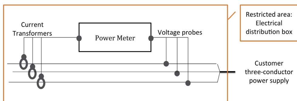
Figure 1. Measuring power with today commercial metering devices.
