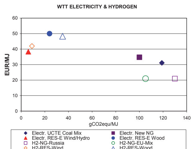
Figure 1b. Electricity and Hydrogen – State of the Art: WTT-emissions [ \text{gCO}_2\text{eq/MJ} ] and production costs as of 2010 [€/MJ]
