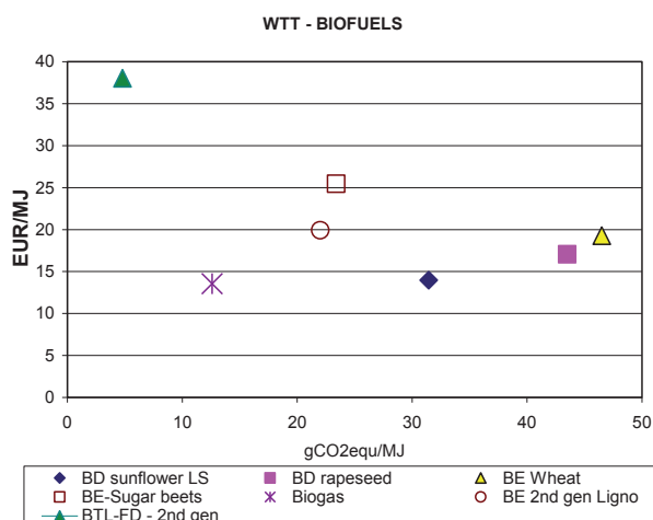
Figure 1a. Biofuels – State of the Art: WTT-emissions [ \text{gCO}_2\text{eq/MJ} ] and production costs as of 2010 [€/MJ]
