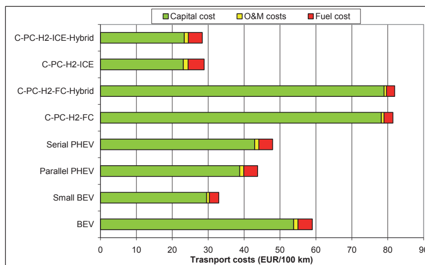
Figure 3. Hydrogen and Electric vehicles – State of the Art of economic assessment of driving costs 2010 (Size of vehicle: 80 kW except small BEV: 47 kW)
