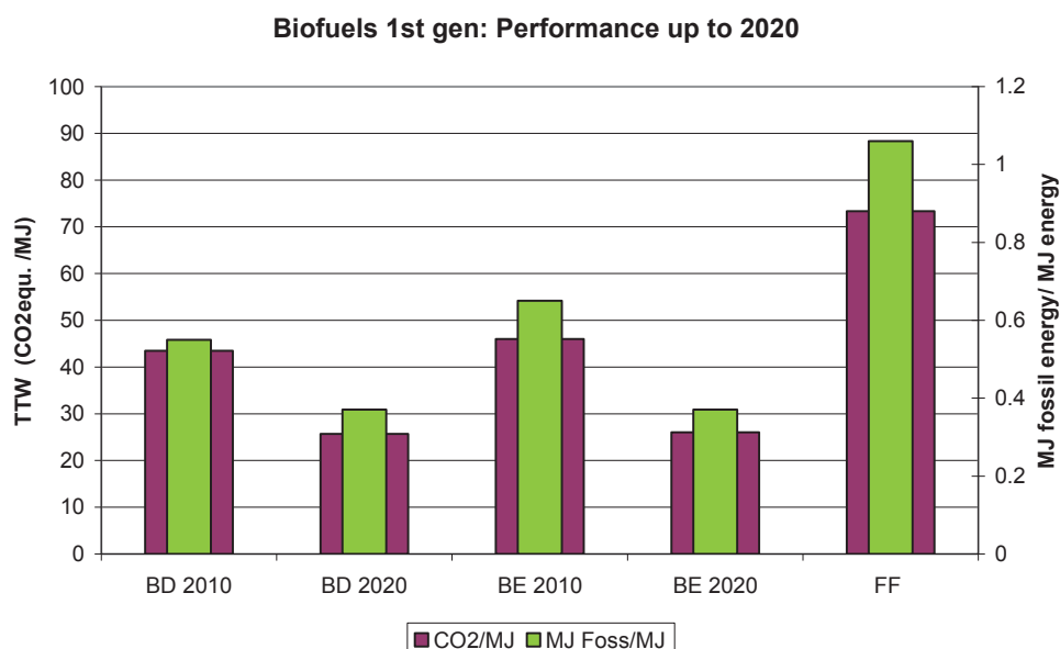
Figure 11. Necessary development of performance of biofuels first generation to meet “Renewable fuel standards” (EC (2008), EC (2009)).
