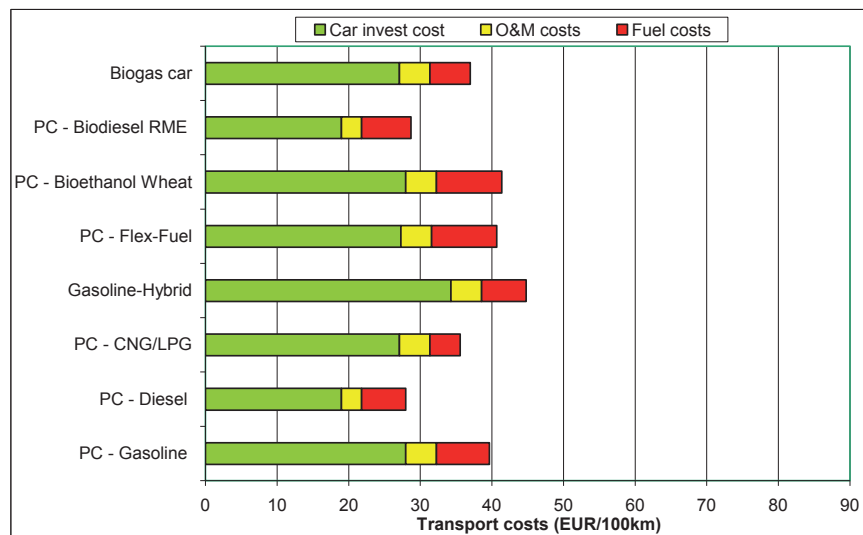
Figure 2. State of the art assessment of driving costs for fossil fuels vs biofuels [€/100km].
