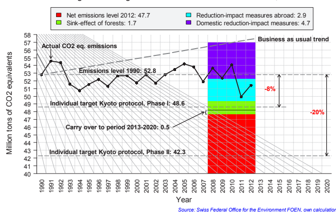
Contributions of greenhouse gas emission reductions in Switzerland, 2008-2012
