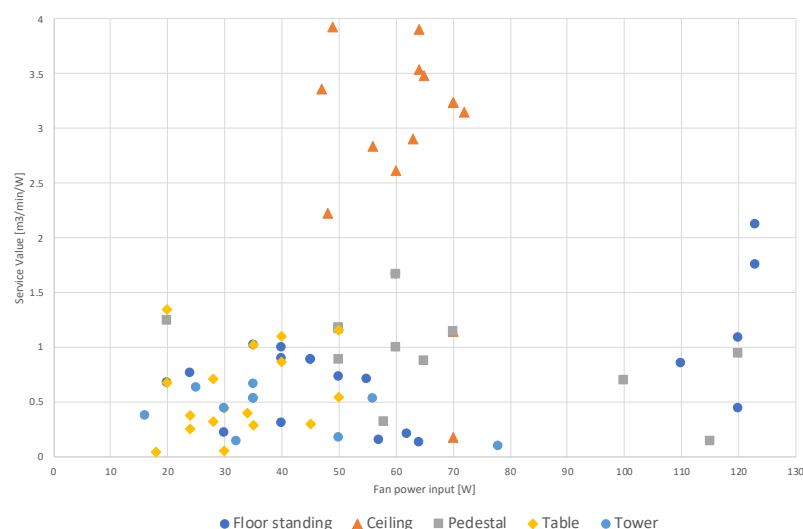
Figure 7. Distribution of fans (according to construction types) according to the Service Value. The Topten selection criteria were based on the service value and selected the 50 % best performing products (data gathered by Topten, 2018).
