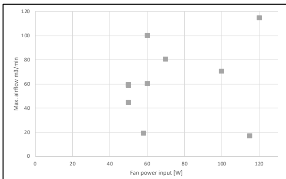
Figure 4. Distribution of pedestal comfort fans according to maximum airflow [m³/min] and fan power input [W] (data gathered by Topten, 2018).
