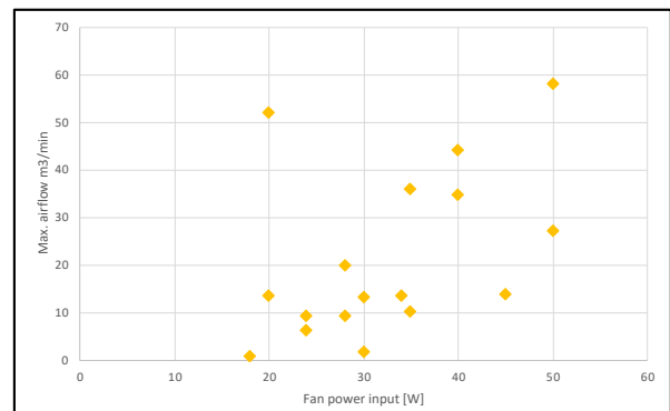
Figure 5. Distribution of table comfort fans according to maximum airflow [m³/min] and fan power input [W] (data gathered by Topten, 2018).
