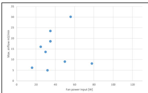
Figure 6. Distribution of tower comfort fans according to maximum airflow [m³/min] and fan power input [W] (data gathered by Topten, 2018).
