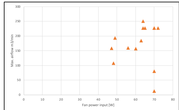
Figure 3. Distribution of ceiling comfort fans according to maximum airflow [m³/min] and fan power input [W] (data gathered by Topten, 2018).
