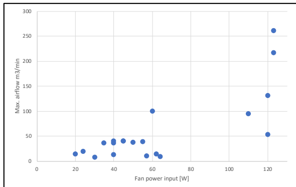
Figure 2. Distribution of floor standing comfort fans according to maximum airflow [m³/min] and fan power input [W] (data gathered by Topten, 2018).
