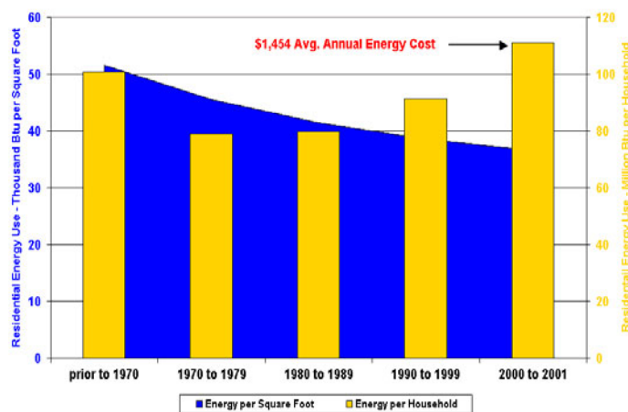
Figure 1. Residential Energy Use by Year of Construction (Site Energy 2 )
