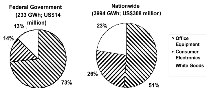
Figure 2. Annual Energy Savings in Year Five.
