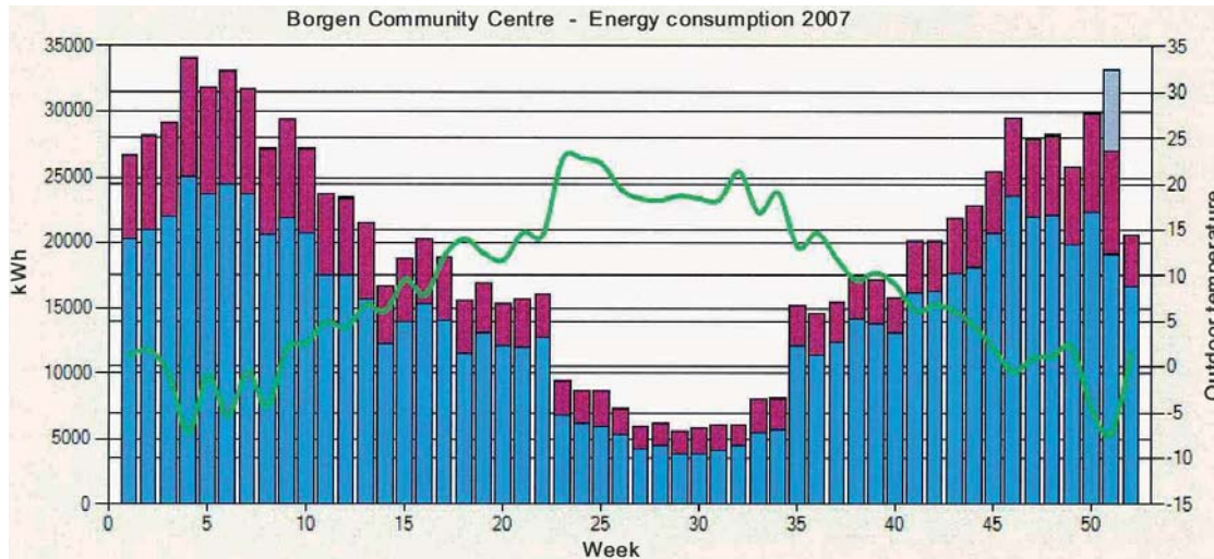
Figure 15. Total energy consumption and mean outdoor temperature in 2007. Blue: Electric power for heating and ventilation. Red: Lighting and appliances. Grey: Oil. Green: Mean outdoor temperature.
