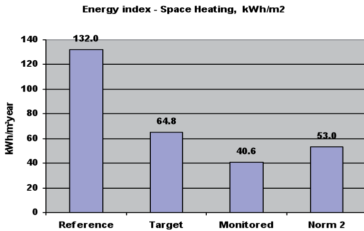
Figure 10. Building energy index.
