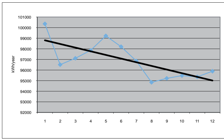
Figure 8. Monitored yearly energy consumption for space heating shown for a 12-month period from October 2006 to October 2007.
